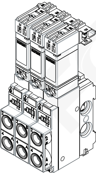
Block installation with extendable valves Cable plug Type 1057
