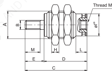
Single acting front spring threaded rod
