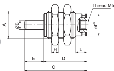
Single acting front spring
