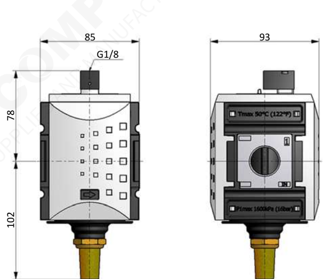
Size Y3, pneumatically operated
