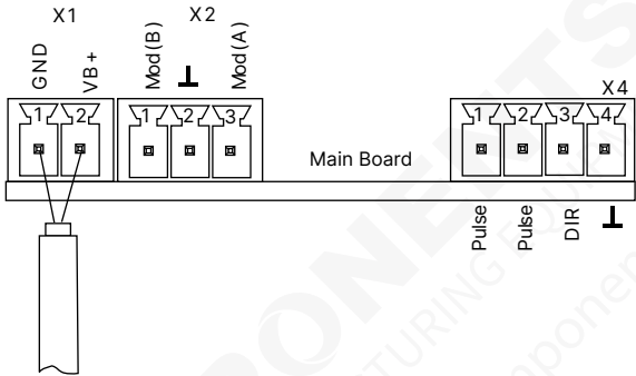
Voltage supply
