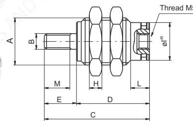
Single acting front spring threaded rod
