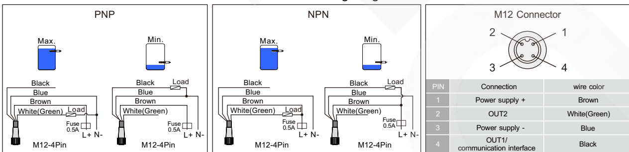
M12x4Pin Wiring Diagram
