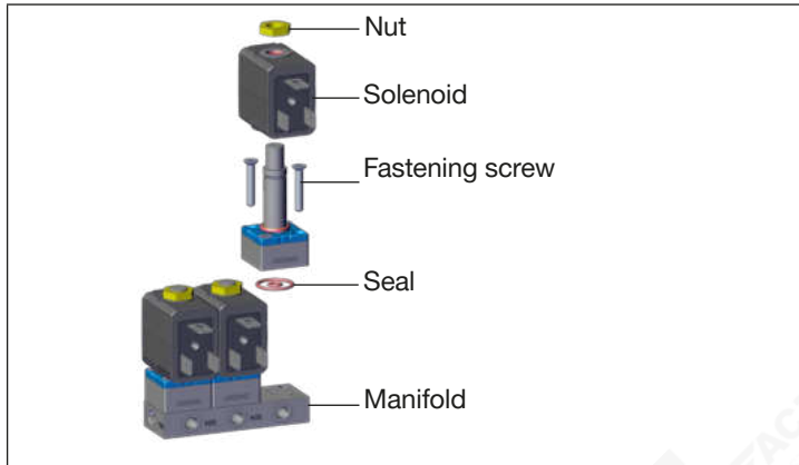
Fig. 3: Installing the devices with a flange connection
